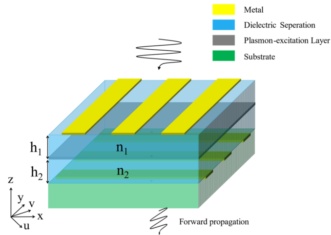
Figure 1. The studied metallic gratings/plasmon-excitation layer/metallic gratings structure.
