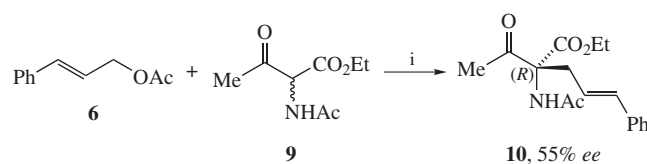
Scheme 5 Reagents and conditions: i, [Pd(\pi\text{-allyl})Cl]_2 , 1 , BSA, KOAc or BSA, Zn(OAc)_2 , PhMe.
