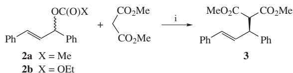
Scheme 2 Reagents and conditions: i, [Pd(\pi\text{-allyl})Cl]_2 (2.0 mol%), 1 (4.0 or 8.0 mol%), 2 (0.25 mmol), dimethyl malonate (1.8 equiv.), BSA (1.8 equiv.), KOAc (8 mol%), solvent (1.5 ml), room temperature, 48 h.
