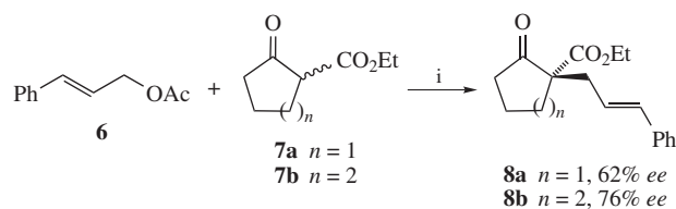
Scheme 4 Reagents and conditions: i, [Pd(\pi\text{-allyl})Cl]_2 , 1 , BSA, Zn(OAc)_2 , PhMe.
