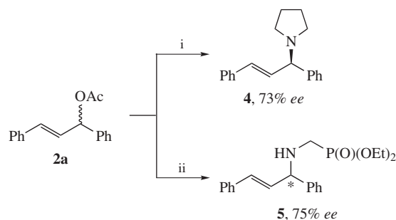
Scheme 3 Reagents and conditions: i, pyrrolidine, [Pd(\pi\text{-allyl})Cl]_2 , 1 , THF; ii, (EtO)_2P(O)CH_2NH_2 , [Pd(\pi\text{-allyl})Cl]_2 , 1 , CH_2Cl_2 .
