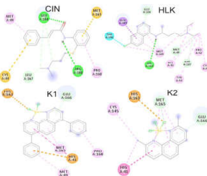
Slika 3. 2D dijagrami nekovalentnih interakcija između proteina i liganda Figure 3. 2D diagrams of non-covalent interactions between protein and ligand
