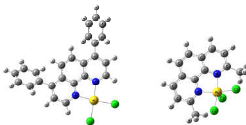
Slika 1. Strukturne formule kompleksa zlata K1 (levo) i K2 (desno) Figure 1. The structures of gold(III) complexes K1 (left) and K2 (right)
