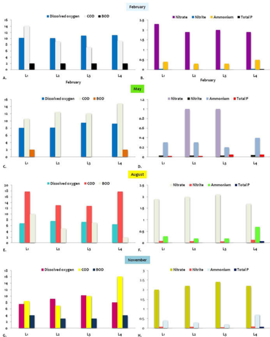
Graph. 2. Seasonal variation of dissolved oxygen ( \text{mg L}^{-1} ), chemical oxygen demand (COD) ( \text{mg L}^{-1} ), biochemical oxygen demand (BOD) ( \text{mg L}^{-1} ), nitrate ( \text{mg L}^{-1} ), nitrite ( \text{mg L}^{-1} ), ammonium ion ( \text{mg L}^{-1} ), total phosphorus ( \text{mg L}^{-1} )
