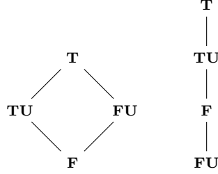
Figure 2. Lattices 4Q and 4LQ .
