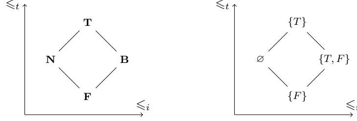
Figure 1. Bilattice \mathcal{FOUR}_2 in Belnap's and generalized truth-values setting.
