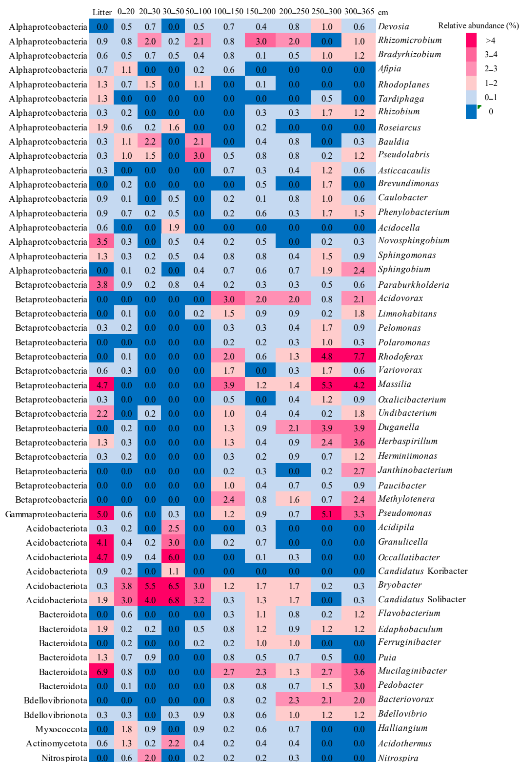
Figure 4. Heatmap of the distribution of 52 most represented cultivated bacterial genera from fen profile samples. The map includes genera the presence of which in at least one out of ten samples exceeds 1%. The numbers in the diagram indicate the percentage of all sequences in the library of 16S rRNA gene fragments (according to SILVA) in each studied sample.
