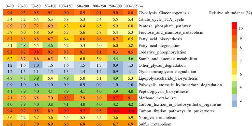
Figure 8. A heatmap showing the clustering of fen profile samples on the relative percentage of iVikodak-derived prokaryotic community functional profiles.
