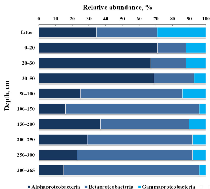
Figure 3. The ratio of classes of the phyla Pseudomonadota in the studied fen profile.
