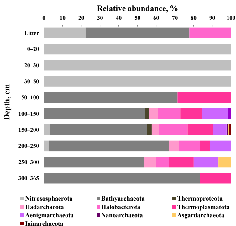
Figure 5. Taxonomic classification of archaeal 16S rRNA gene fragments in the libraries from fen profile samples at the phyla level.
