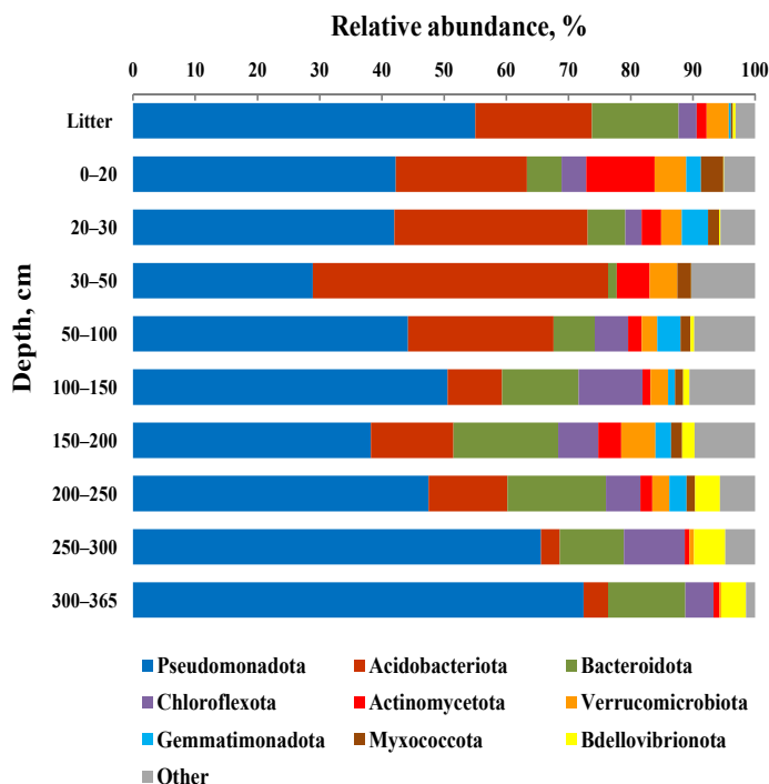
Figure 2. Taxonomic classification of bacterial 16S rRNA gene fragments in the libraries from fen profile samples at the phylum level. The list includes taxa constituting >3% in each library.
