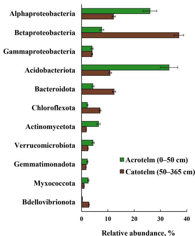
Figure 7. Relative proportion of bacterial 16S rRNA gene fragment sequences represented at the phyla level (at the class level for Pseudomonadota) in libraries from acrotelm and catotelm samples of the studied fen profile. The mean values are given for nine acrotelm horizons and eighteen catotelm horizons. Error bars indicate the standard error of means.
