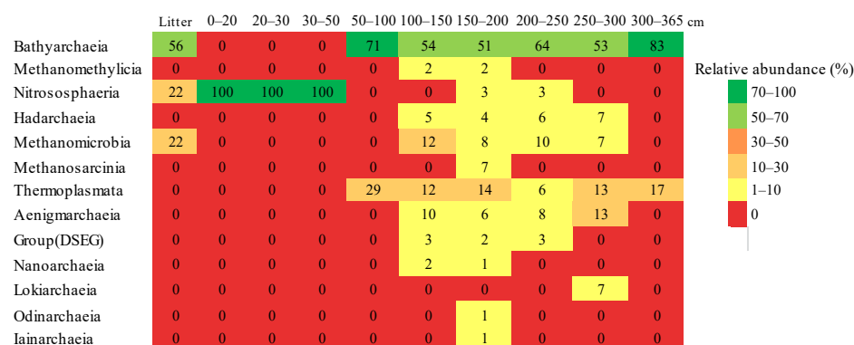
Figure 6. A heatmap showing the clustering of fen profile samples on the relative abundance of archaeal 16S rRNA gene sequences represented at the class level.
