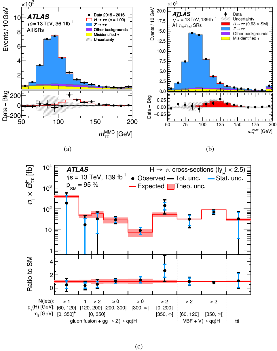
Fig. 12. (a) The invariant mass of the \tau\tau system for all combinations of \tau -lepton decays using 36.1 \text{fb}^{-1} of data [123]. (b) The same observable considering only signal regions with one \tau -lepton decaying leptonically and one decaying hadronically for 139 \text{fb}^{-1} of data [125]. (c) The measured cross-sections times branching ratio in nine different kinematic regions compared with the SM expectations [125].
