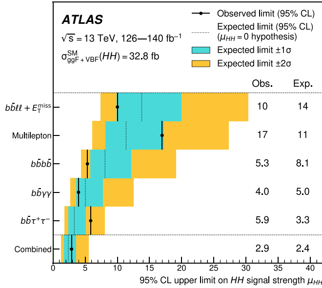
Fig. 32. Observed and expected 95% CL upper limits on \mu_{HH} for double Higgs boson production in the HH \rightarrow b\bar{b}\ell\ell + E_T^{\text{miss}} , multilepton, HH \rightarrow b\bar{b}\gamma\gamma , HH \rightarrow b\bar{b}\tau^+\tau^- and HH \rightarrow b\bar{b}b\bar{b} decay channels and their statistical combination [193]. The expected limit is derived assuming \mu_{HH} = 0 .
