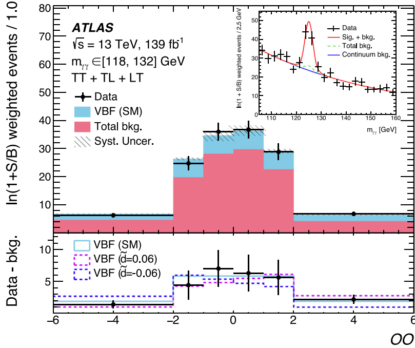
Fig. 28. Distribution of the Optimal Observable in the H \rightarrow \gamma\gamma decay channel, for events enriched in the VBF production mode, with 118 < m_{\gamma\gamma} < 132 GeV [174]. The total background includes events from non-VBF Higgs production. The bottom panel contains the background-subtracted distribution for data as well as the prediction for the SM and for two non-zero values of \tilde{d} . The invariant mass distribution is shown in the inset on the top right. Category-dependent weights are applied.
