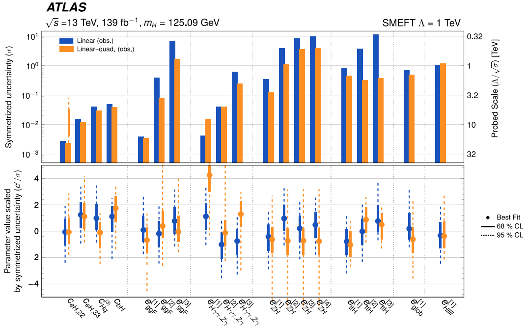
Fig. 27. Comparison of the observed parameters of the rotated basis with the SMEFT model that keeps only terms linear in the new operators (blue) and the model including quadratic terms (orange), where all other coefficients and nuisance parameters are profiled, i.e., set to the values that maximise the likelihood [158]. The top panel shows the symmetrised 68% CL uncertainty \sigma of each parameter measurement (left vertical axis) and the corresponding energy scale \Lambda/\sqrt{\sigma} , \Lambda = 1 TeV that is probed (right vertical axis). The bottom panel shows the measured parameter value, 68% (solid) and 95% (dashed) CL intervals, divided by the symmetrised uncertainty shown in the top panel.
