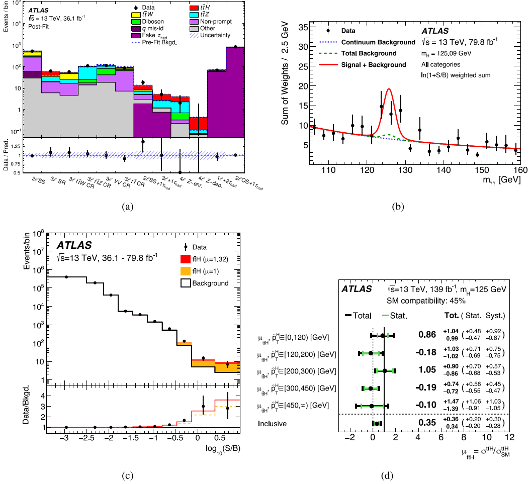
Fig. 13. (a) Comparison of the data to the prediction in the different signal and control regions of the t\bar{t}H , H \rightarrow multilepton analysis, after the fit is performed [129]. (b) The diphoton invariant mass distribution in the t\bar{t}H , H \rightarrow \gamma\gamma analysis [126]. (c) Event yields as a function of \log_{10}(S/B) for data, background and a Higgs boson signal for all decay channels considered, using up to 79.8 \text{ fb}^{-1} of data, leading to the observation of t\bar{t}H production [126]. (d) Measured t\bar{t}H production cross-sections normalised to the SM expectation as function of p_T^H in the H \rightarrow b\bar{b} final state [130].
