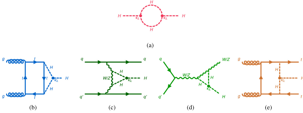
Fig. 33. Examples of one-loop \lambda_{HHH} -dependent diagrams for (a) the Higgs boson self-energy, and for single Higgs boson production in the (b) ggF, (c) VBF, (d) VH, and (e) t\bar{t}H modes. The self-coupling vertex is indicated by the filled circle [197].
