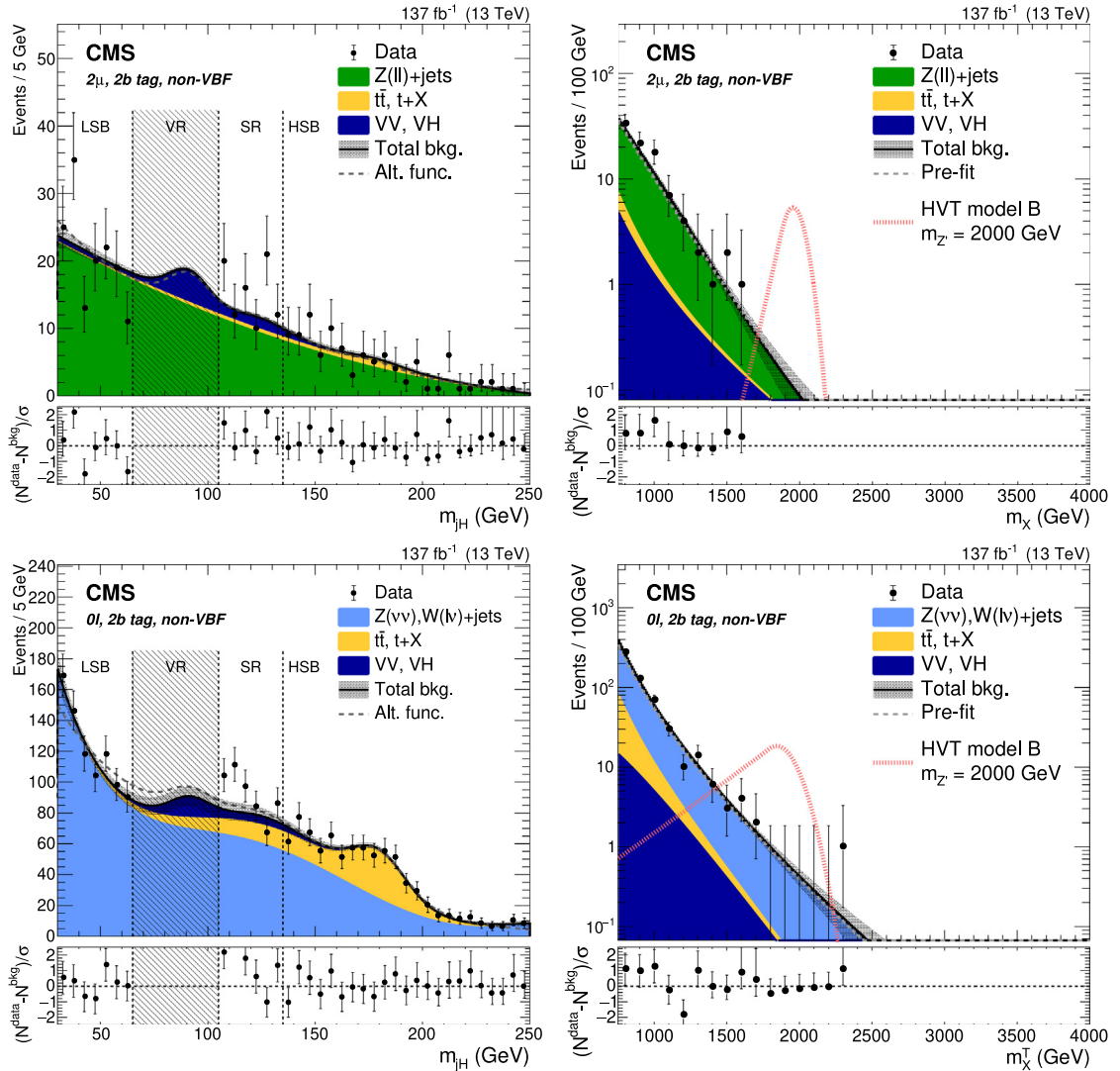
Fig. 16. Search for X \rightarrow V H(bb) : Distributions of (left) the jet soft drop mass of a boosted Higgs boson candidate, labeled m_{jH} , and (right) the mass or transverse mass of the X resonance candidate, labeled m_X and m_X^T , respectively, in the Z(\ell\ell)H(bb) (upper) and Z(vv)H(bb) channels (lower). The shaded area depicts a veto region excluded from the analysis to minimize the event overlap with dedicated searches in the VV decay channel. Source: Figures from Ref. [117].
