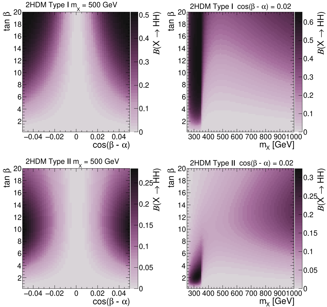
Fig. 5. Branching fractions of X \rightarrow HH decays in 2HDMs of Type I (upper) and Type II (lower) in the \cos(\beta - \alpha) - \tan \beta plane for m_X = 500 GeV (left) and in the m_X - \tan \beta plane for \cos(\beta - \alpha) = 0.02 (right). The masses of all non-SM-like Higgs bosons are set to be the same, m_X = m_A , and m_{12}^2 = m_A^2 \tan \beta / (1 + \tan^2 \beta) . The branching fractions have been calculated with 2HDMC v1.8.0 [62,63].
