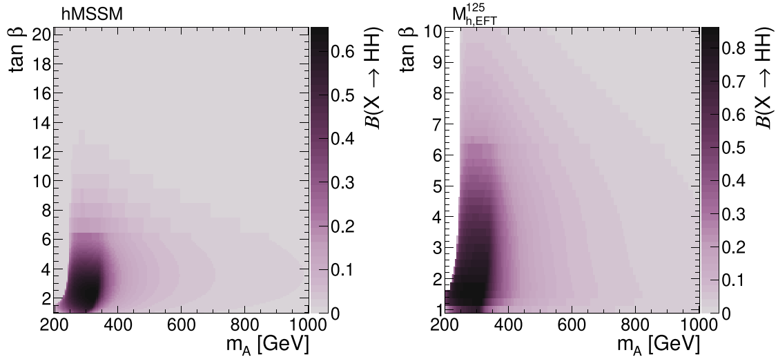
Fig. 6. Branching fraction of X \rightarrow HH decays in the MSSM, for the hMSSM [64–66] (left) and the M_{h,EFT}^{125} [67] benchmarks, in the m_A – \tan \beta plane. Source: The branching fractions are taken from benchmark files produced by the MSSM subgroup of the LHC Higgs Working Group [68,69].
