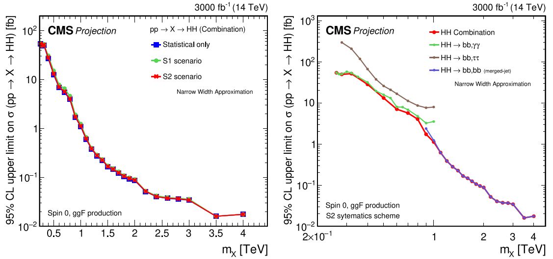
Fig. 45. Expected upper limits at 95% CL, on the product of the cross section for the production of a spin-0 resonance X and the branching fraction \mathcal{B}(X \rightarrow HH) , as a function of m_X , for an integrated luminosity of 3000 \text{ fb}^{-1} and the combination of the three analyses shown in Fig. 44. Shown are the effects of the different systematic uncertainty scenarios (left), and the reach of the individual analyses for the S2 systematic scenario (right). All estimates include the anticipated statistical uncertainties.
