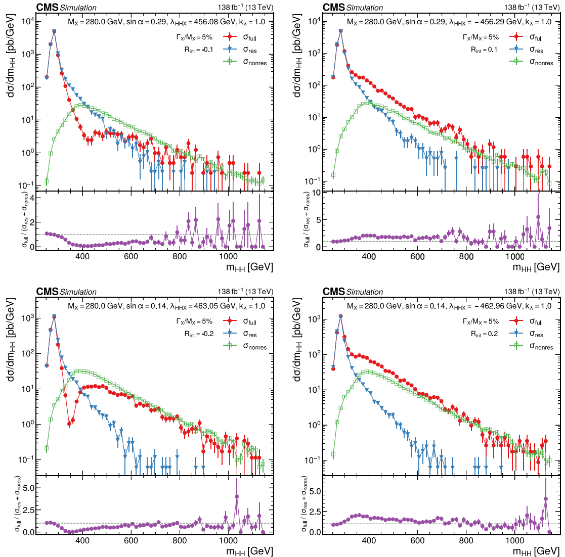
Fig. 42. Expected differential cross sections for HH production, as a function of m_{HH} , for the real-singlet model with m_X = 280\text{ GeV} and \Gamma_X/m_X = 5\% . The parameters \sin\alpha and \lambda_{HHX} have been chosen such that (upper row) R_{\text{int}} = \pm 10\% and (lower row) R_{\text{int}} = \pm 20\% , for (left) negative and (right) positive values of R_{\text{int}} . The total cross section for HH production \sigma^{\text{full}} (red line, labeled as \sigma_{\text{full}} ) is compared to the cross sections \sigma^{\text{resonant-only}} (blue line, labeled as \sigma_{\text{res}} ) and \sigma^{\text{nonresonant}} (green line, labeled as \sigma_{\text{nonres}} ) considering only resonant and nonresonant production. In the lower panels the ratio of \sigma^{\text{full}} over (\sigma^{\text{resonant-only}} + \sigma^{\text{nonresonant}}) is shown.
