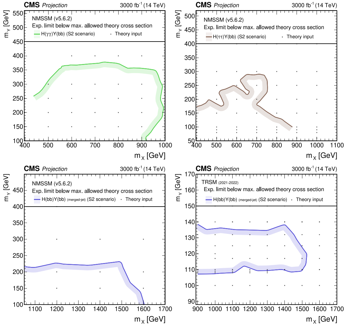
Fig. 53. Interpretation of the upper limits at 95% CL, on the product of the cross section \sigma for the production of a resonance X via gluon-gluon fusion and the branching fraction B for the X \rightarrow Y(bb)H decay, obtained from the projections to an integrated luminosity of 3000 \text{ fb}^{-1} of the (upper left) Y(bb)H(\gamma\gamma) [123], (upper right) Y(bb)H(\tau\tau) [122], and (lower row) Y(bb)H(bb) [124] analyses, assuming the S2 systematic uncertainty scenario. The projected limits are mapped onto the (m_X, m_Y) plane, and compared with the maximally allowed cross sections of the NMSSM (left and upper right), and TRSM models (lower right) discussed in Section 4.1.3. The points indicate the available theory predictions. The mass dependences of both the projected experimental limits and the maximally allowed theory cross sections have been interpolated to obtain approximate exclusion contours. The NMSSM predictions based on NMSSMTools version 5.6.2 are adapted from Ref. [200], whereas the TRSM is described in Ref. [12]. In both cases, the model predictions have been scaled to \sqrt{s} = 14 \text{ TeV} .
