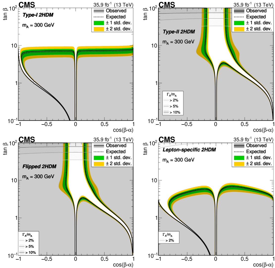
Fig. 33. Interpretation of the results of the A \rightarrow ZH(bb) analysis [115], in the (upper left) Type I, (upper right) Type II, (lower left) flipped, and (lower right) lepton-specific 2HDM models. In each case observed and expected exclusion contours at 95% CL, in the plane defined by \cos(\beta - \alpha) and \tan \beta , are shown. The excluded regions are represented by the shaded gray areas. The 68 and 95% central intervals of the expected exclusion contours in the absence of a signal are indicated by the green and yellow bands. Contours are derived from the projection on the corresponding 2HDM parameter space for m_A = 300 GeV. The regions of parameter space where the natural width of the A boson \Gamma_A is comparable to or larger than the experimental resolution and thus the narrow-width approximation is not valid are represented by hatched gray areas. Source: Figure from Ref. [115].
