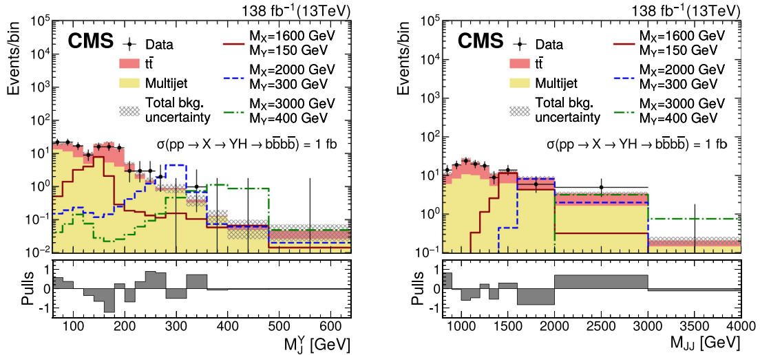
Fig. 23. Search for X \rightarrow Y(bb)H(bb) : Distributions of the (left) soft-drop mass of the boosted Y candidate, labeled M_J^Y , and (right) the dijet mass of the Y and H candidates, M_{JJ} , in the high-purity SR of the Y(bb)H(bb) analysis with two merged bb jets [124]. The distributions as expected for signals with three different values of m_X and m_Y (labeled M_X and M_Y ) are also shown. In the lower panels the statistical pull in each bin is displayed.
