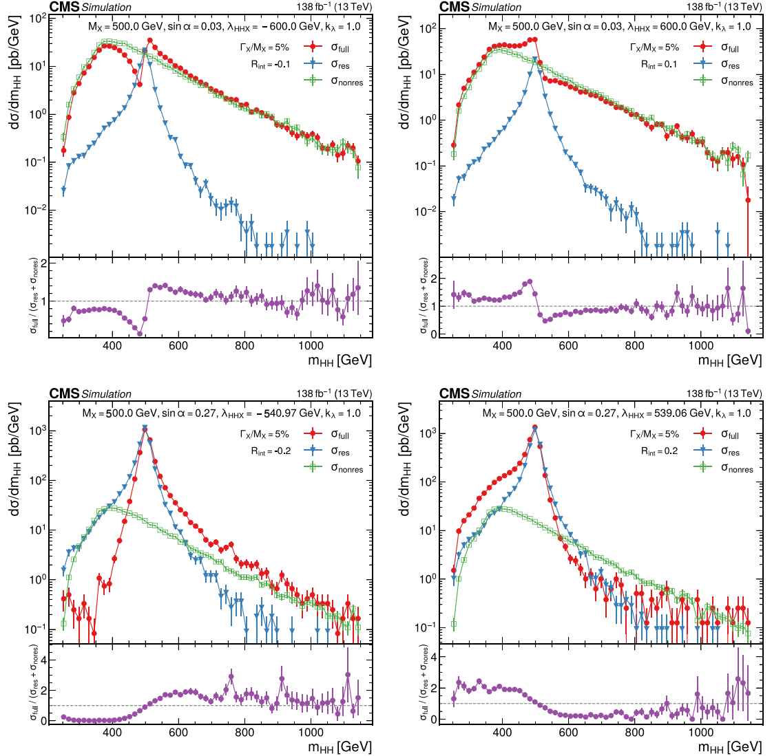
Fig. 43. Expected differential cross sections for HH production, as a function of m_{HH} for the real-singlet model with m_X = 500 GeV and \Gamma_X/m_X = 5\% . The parameters \sin \alpha and \lambda_{HHX} have been chosen such that (upper row) R_{\text{int}} = \pm 10\% and (lower row) R_{\text{int}} = \pm 20\% , for (left) negative and (right) positive values of R_{\text{int}} . The total cross section for HH production \sigma_{\text{full}} (red line, labeled as \sigma_{\text{full}} ) is compared to the cross sections \sigma_{\text{resonant-only}} (blue line, labeled as \sigma_{\text{res}} ) and \sigma_{\text{nonresonant}} (green line, labeled as \sigma_{\text{nonres}} ) considering only resonant and nonresonant production. In the lower panels the ratio of \sigma_{\text{full}} over (\sigma_{\text{resonant-only}} + \sigma_{\text{nonresonant}}) is shown.
